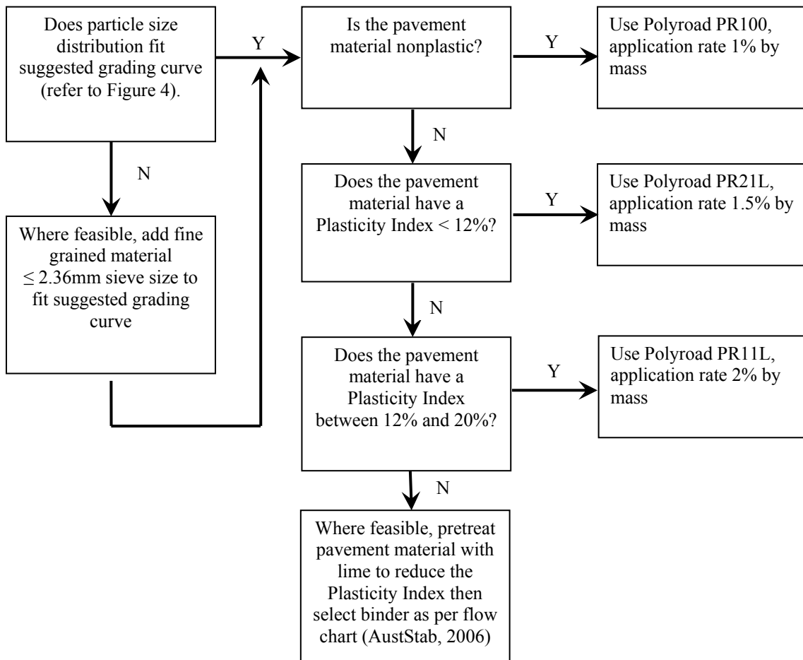
Figure 3 Determination of Polyroad binders for granular pavement materials.
