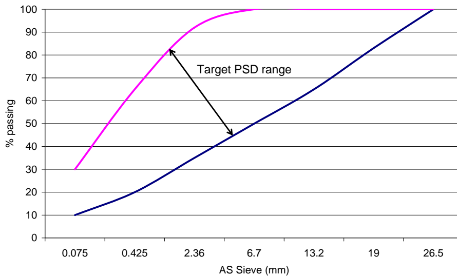
Figure 4 Suggested particle distribution range for Polyroad binders.
